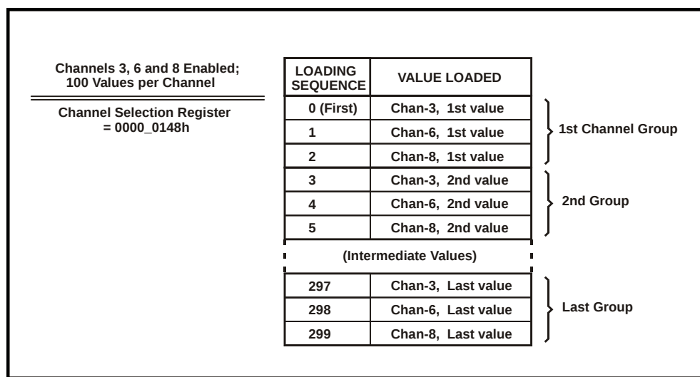
Figure 3.4-1. Typical Buffer Loading Sequence
