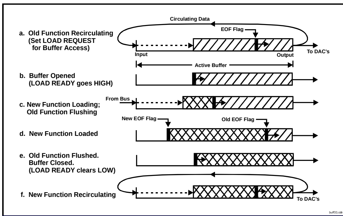
Figure 3.4-4. Function Sequencing
