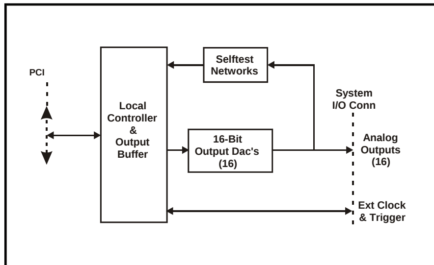
Figure 1.2-1. Functional Organization
