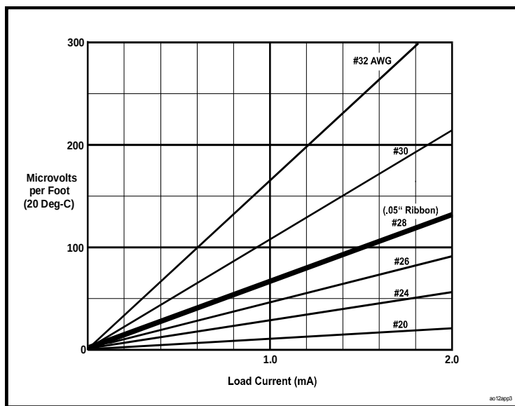
Figure 2.3-2. Line Loss Versus Load Current
