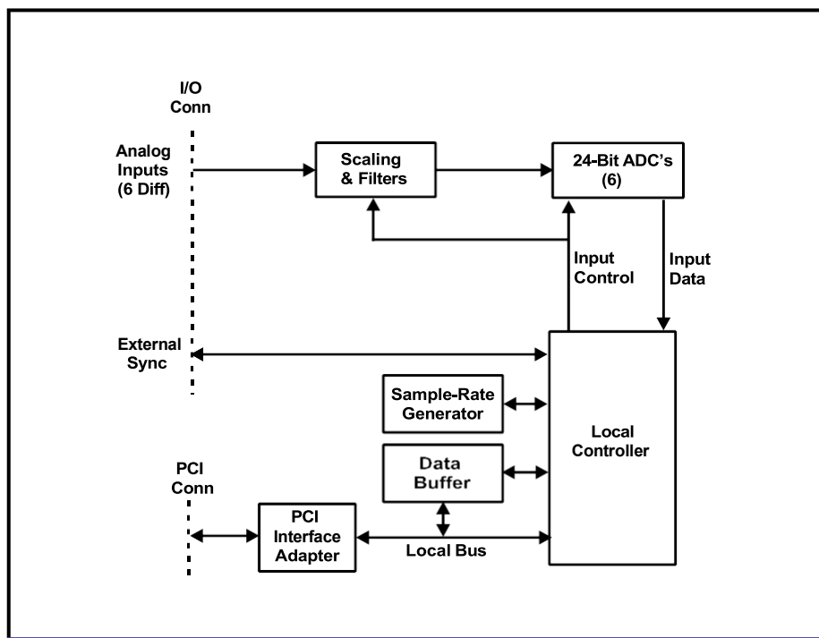
Figure 1.2. Functional Organization
