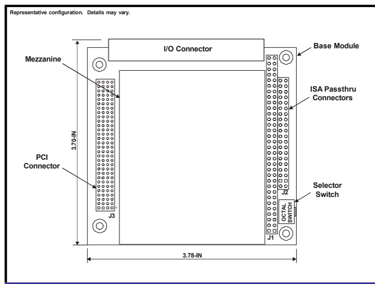
Figure 1.1. Physical Configuration
