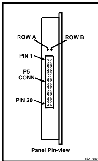
Figure 2.2.2. System Input/Output Connector
