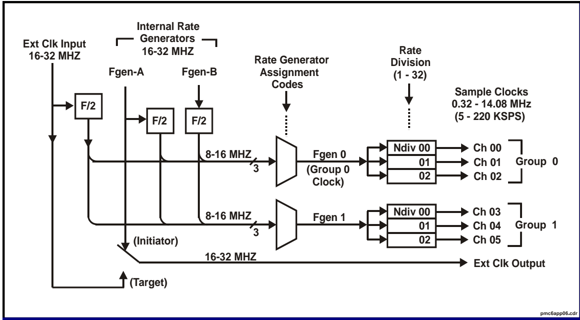
Figure 3.6.1.1. Rate Clocks Organization, 6-Channel Board
