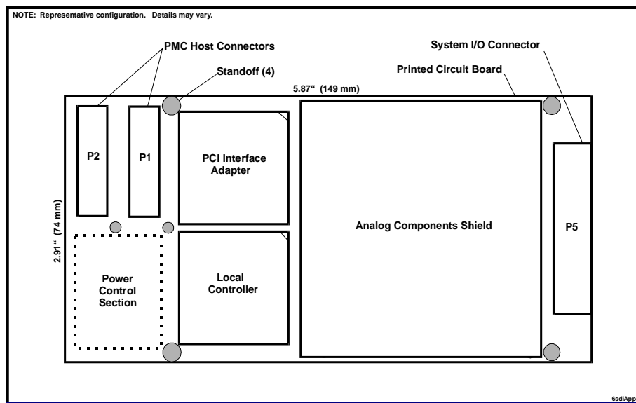
Figure 1.1. Physical Configuration
