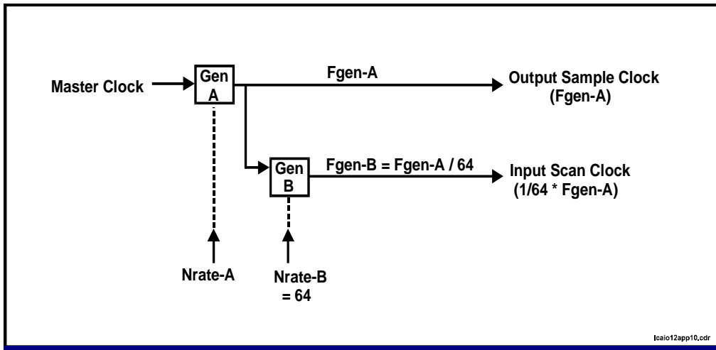
Figure 3.4-2. Cascaded Rate Generator Example
