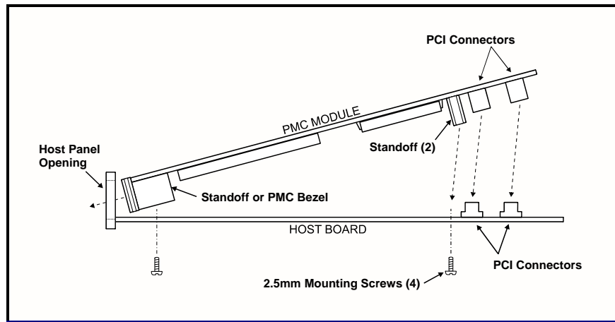
Figure 2.2-1. Physical Installation
