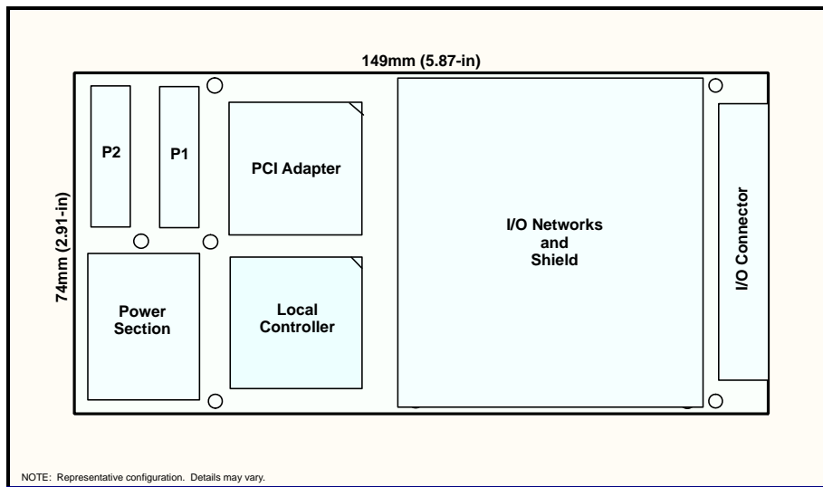
Figure 1.1-1. Physical Configuration
