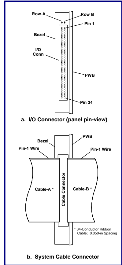
Figure 2.2-2. Input/Output Connector
