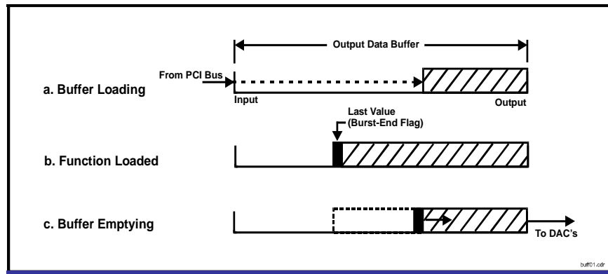
Figure 3.6-1. Function Burst; Output Buffer Data Flow
