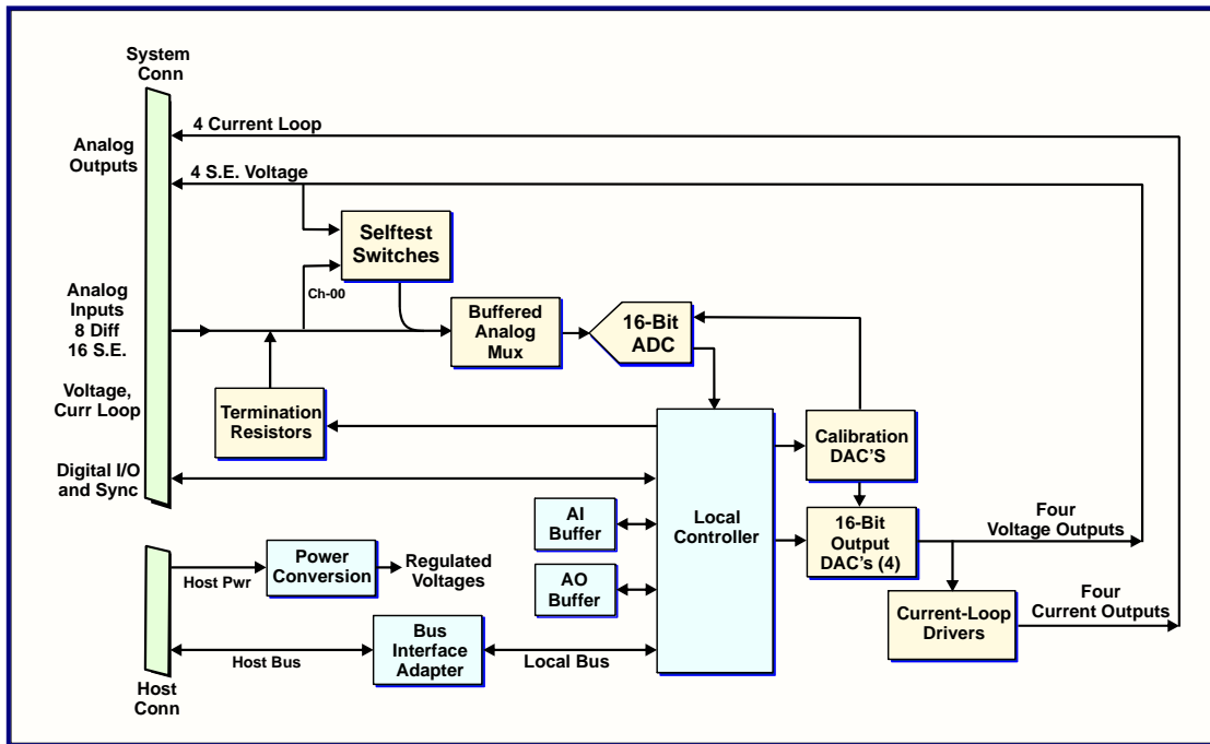
Figure 1.2-1. Functional Organization
