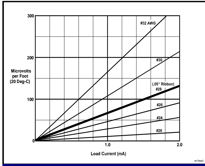
Figure 2.3-3. Line Loss Versus Load Current
