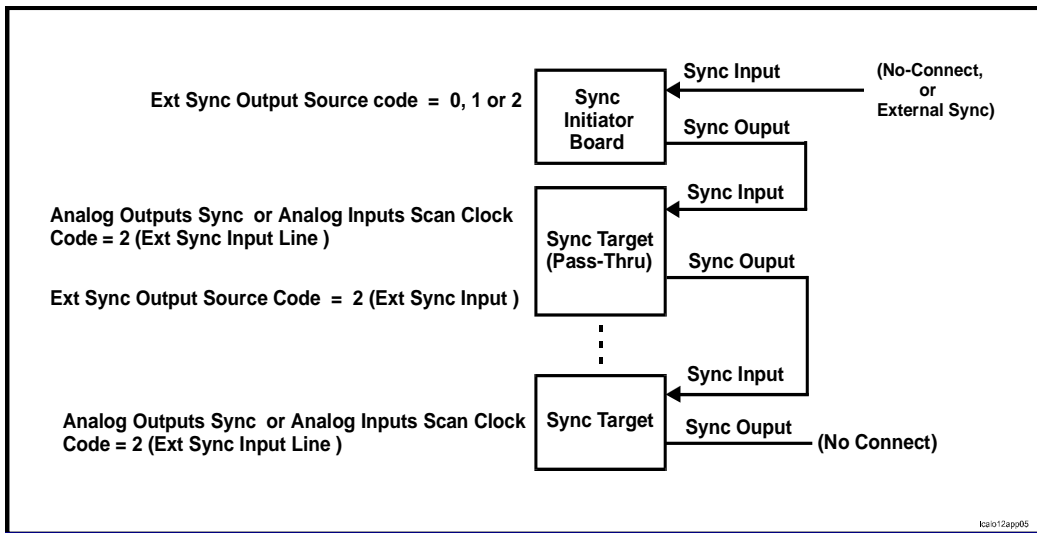
Figure 3.5-1. Multiboard Synchronization
