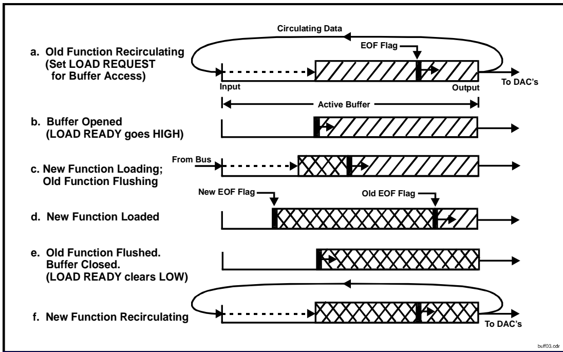
Figure 3.4-4. Function Sequencing
