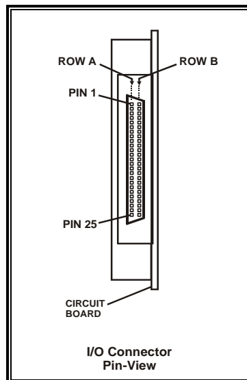
Figure 2.2.2. System Input/Output Connector
