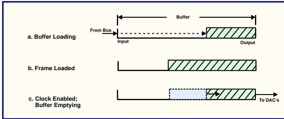
Figure 3.4-1. Open Buffer Data Flow
