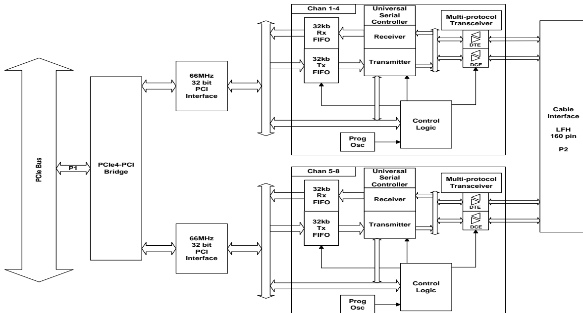
Figure 1-1 Block Diagram of PCIe4-SIO8BX2
