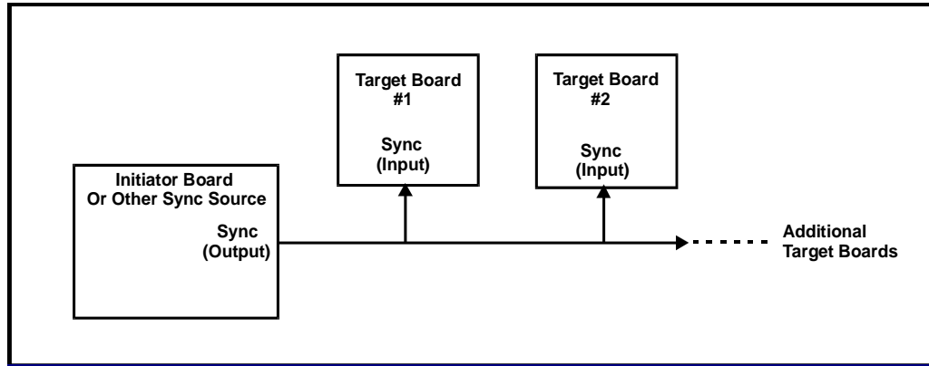
Figure 2.3-2. Multiboard Synchronization
