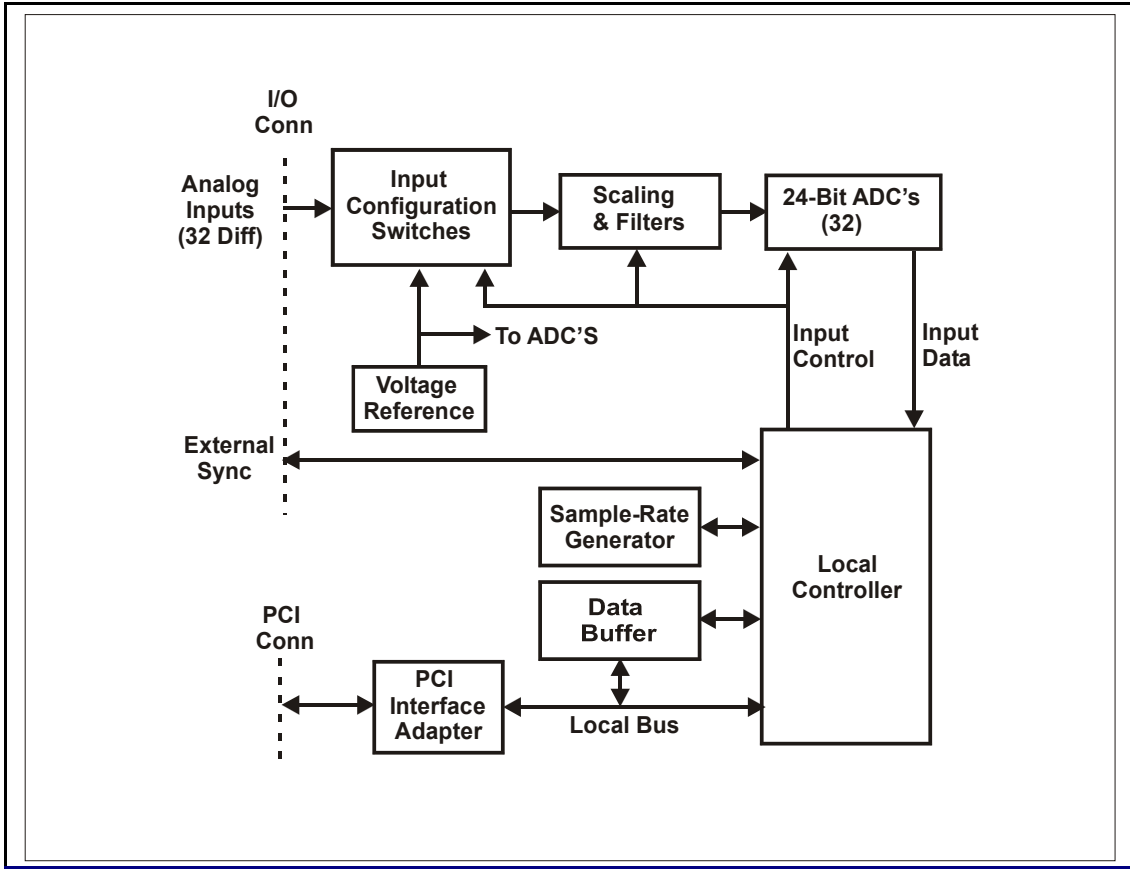
Figure 1. cPCI6U-24DSI32R; Functional Organization
