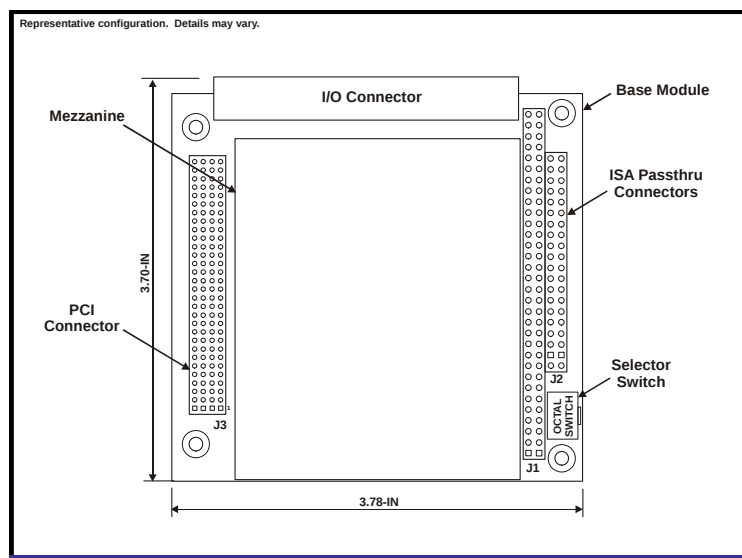
Figure 1.1. Physical Configuration
